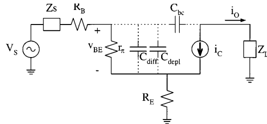
Fig. 1. HBT equivalent circuit with dotted capacitances for a high-frequency operation.
