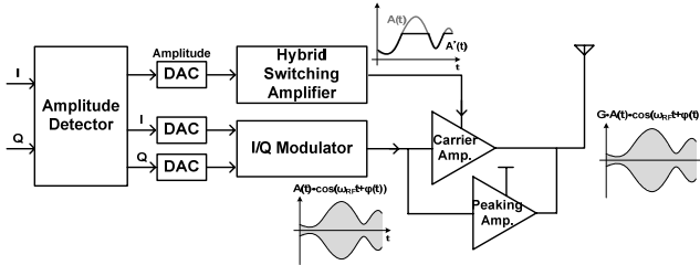
Fig. 5. Block diagram of envelope tracking Doherty PA [24]
