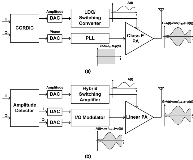
Fig. 4. Block diagram of (a) conventional polar transmitter and (b) advanced polar transmitter – envelope tracking PA [22]
