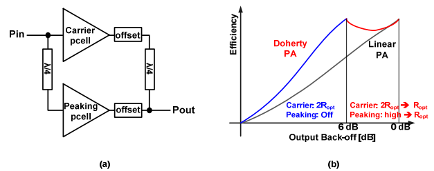
Fig. 3. (a) Block diagram of Doherty PA and (b) operation principle
