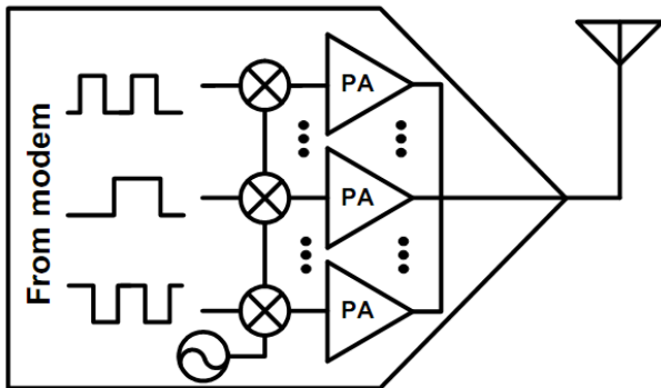
Fig. 7. All digital transmitter architecture
