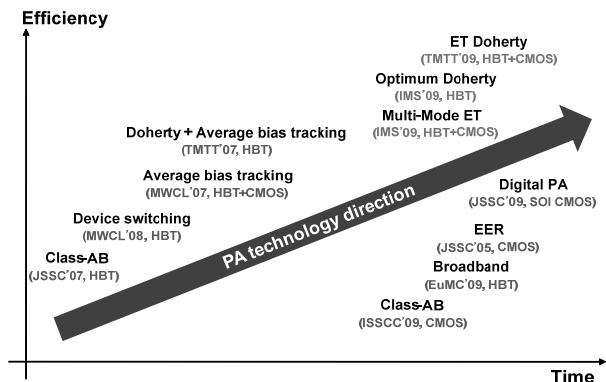
Fig. 2. Recent PA technology direction based on Fig. 1
