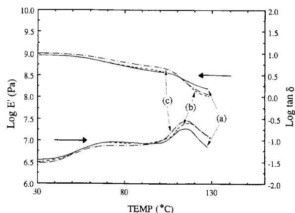
Figure 6 Plots of storage modulus ( E' ) and loss tangent ( \tan \delta ) versus temperature for 75/25 PBT/PS blends with various amounts of PS-GMA: (a) 0 phr; (b) 5 phr; (c) 10 phr
