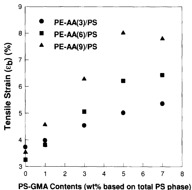
Figure 8 Change in elongation at break ( \epsilon_b ) with PS-GMA content for three different PE-AAs/PS blends: (●) PE-AA(3)/PS; (■) PE-AA(6)/PS; (▲) PE-AA(9)/PS. All blend compositions are 30/70 (wt/wt) PE-AA/PS
