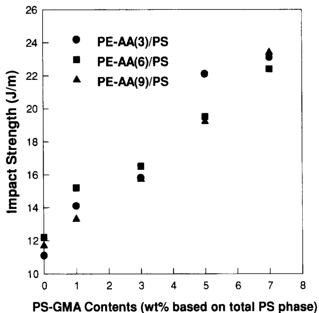
Figure 11 Change in Izod impact strength with PS-GMA content for three different PE-AAs/PS blends: (●) PE-AA(3)/PS; (■) PE-AA(6)/PS; (▲) PE-AA(9)/PS. All blend compositions are 30/70 (wt/wt) PE-AA/PS
