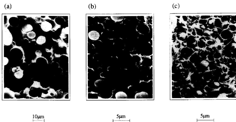
Figure 1 Morphologies of fractured surfaces for 30/70 (wt/wt) PE-AA(3)/PS blends with three different amounts of PS-GMA (wt% in total PS phase): (a) 0; (b) 3; (c) 7
