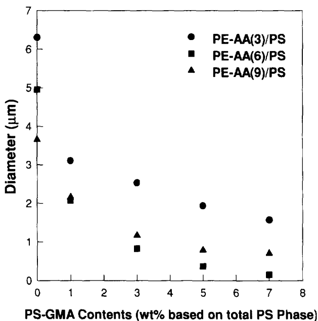
Figure 4 Plots of the number average domain size ( D_n ) vs the amount of PS-GMA for three different PE-AA/PS blends: (●) PE-AA(3)/PS; (■) PE-AA(6)/PS; (▲) PE-AA(9)/PS. All blend compositions are 30/70 (wt/wt) PE-AA/PS
