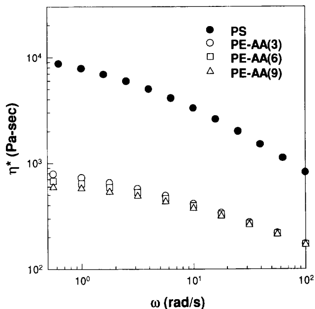
Figure 6 Complex viscosity ( \eta^*(\omega) ) vs frequency ( \omega ) for three different PE-AA copolymers and neat PS at 210°C: (○) PE-AA(3); (□) PE-AA(6); (△) PE-AA(9); (●) PS
