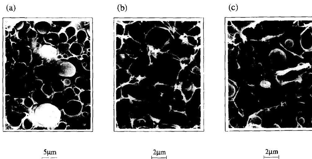
Figure 3 Morphologies of fractured surfaces for 30/70 (wt/wt) PE-AA(9)/PS blends with three different amounts of PS-GMA (wt% in total PS phase): (a) 0; (b) 3; (c) 7
