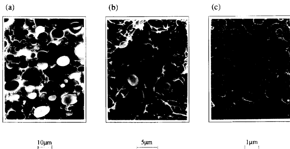
Figure 2 Morphologies of fractured surfaces for 30/70 (wt/wt) PE-AA(6)/PS blends with three different amounts of PS-GMA (wt% in total PS phase): (a) 0; (b) 3; (c) 7
