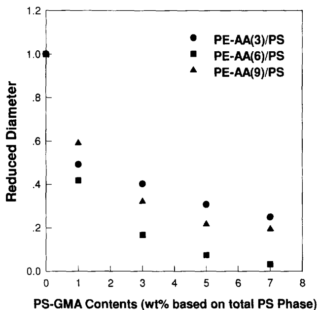
Figure 5 Plots of the reduced domain size ( D_r ) vs the amount of PS-GMA for three different PE-AA/PS blends: (●) PE-AA(3)/PS; (■) PE-AA(6)/PS; (▲) PE-AA(9)/PS. All blend compositions are 30/70 (wt/wt) PE-AA/PS
