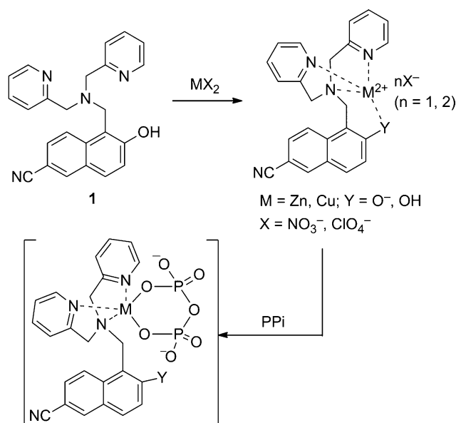
Fig. 1 Schematic presentation of the Zn(II) and Cu(II) complexes of dipicolylamine-hydroxynaphthalene 1 , and their PPI-bound complexes.
