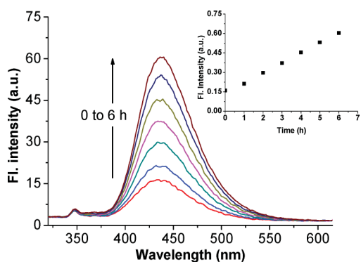
Fig. 5 Time-dependent fluorescence enhancement of 1-Zn(II) ( 10\ \mu\text{M} ) in the presence of 100 equiv. of PPI in 10 mM HEPES buffer of pH 7.4 (excitation at 310 nm). Inset: a plot of fluorescence intensity change with time (intensity was estimated by the peak height at \lambda = 435\ \text{nm} ).
