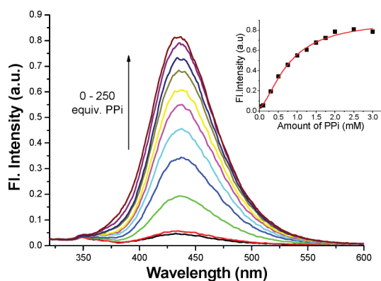
Fig. 4 Fluorescence titration of 1-Zn(II) ( 10\ \mu\text{M} ) against PPI in 10 mM HEPES buffer of pH 7.4, measured 6 h after addition of analyte (excitation at 310 nm; intensity was estimated by the peak height at \lambda = 435\ \text{nm} ).
