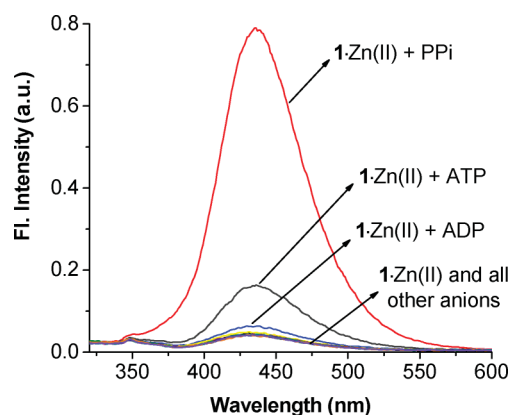
Fig. 3 Fluorescence response of 1-Zn(II) ( 10\ \mu\text{M} ) toward each of various anions (200 equiv.; PPI, ATP, ADP, 1-Zn(II) , \text{H}_2\text{PO}_4^{2-} , \text{AcO}^- , \text{PO}_4^{3-} , \text{HSO}_4^- , \text{ClO}_4^- , \text{F}^- , \text{Cl}^- , \text{Br}^- , \text{I}^- , \text{NO}_2^- and \text{NO}_3^- respectively) as their sodium salts in a HEPES buffer (10 mM, pH 7.4); measured after 6 h upon addition of the anion (excitation at 310 nm; intensity was estimated by the peak height at \lambda = 435\ \text{nm} ).
