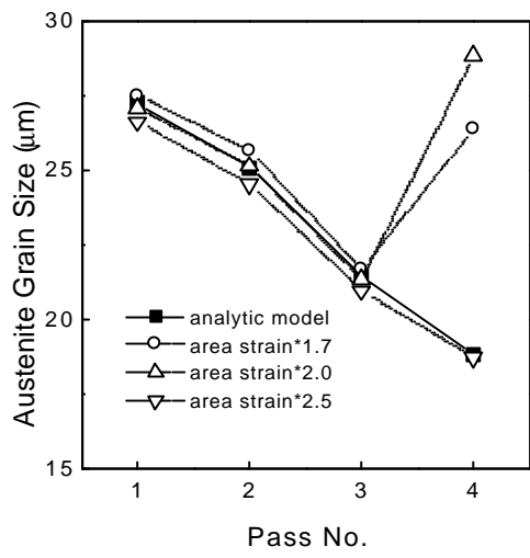
Fig. 5 Predicted AGS and measured one during the four pass rolling sequence.
