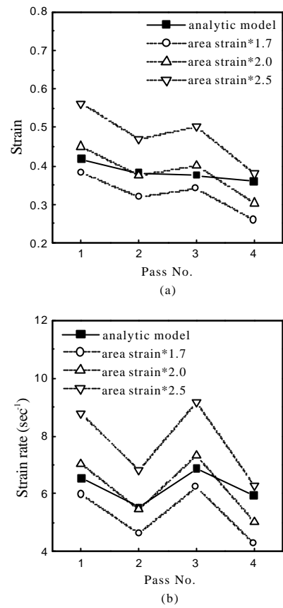
Fig. 2 Comparison of deformation parameters calculated by the analytic and area strain model when the finishing rolling speed is 1[m/s]. (a) Strains and (b) Strain rates
