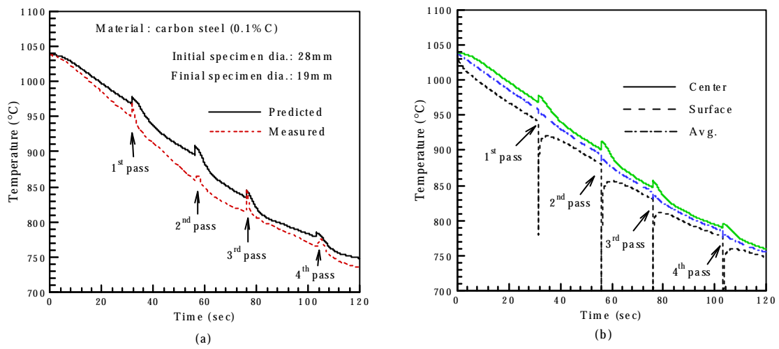
Fig. 3 Time - temperature history of workpiece during the four-pass bar rolling (a) Predicted and measured centerline temperature of specimen and (b) Predicted temperature across the cross section of specimen
