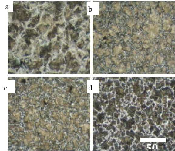
Fig. 6 The measured austenite grains for the four-pass bar rolling sequence. (a) 1 st pass (b) 2 nd pass (c) 3 rd pass and (d) 4 th pass.
