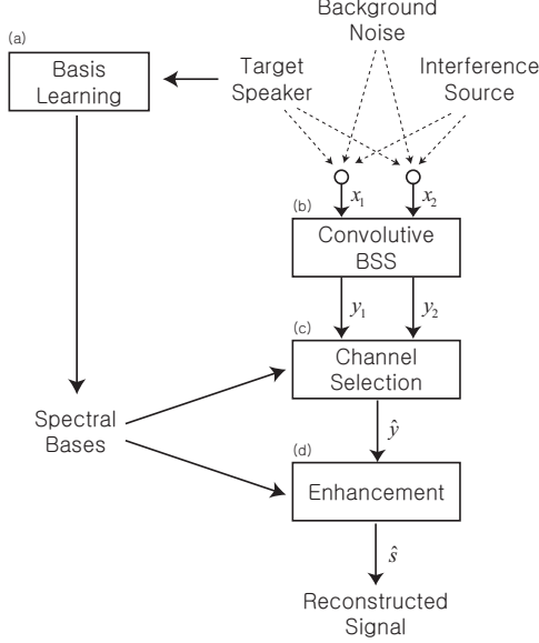
Fig. 1. The schematic diagram of our proposed method for target speech extraction is shown: (a) learning spectral bases given training utterances described in Sec. 3; (b) convolutional BSS to restore independent sources from convolutional mixtures, where we used methods exploiting nonstationarity [13, 14, 6]; (c) channel selection takes two outputs y_1 and y_2 (outputs of BSS) as inputs to identify the source corresponding to the target speaker, yielding an estimate of target speech, \hat{y} , described in Sec. 4.1; (d) enhancement where we suppress the interference and noise remaining in \hat{y} , yielding the final estimate \hat{s} of target speech, described in Sec. 4.2.
